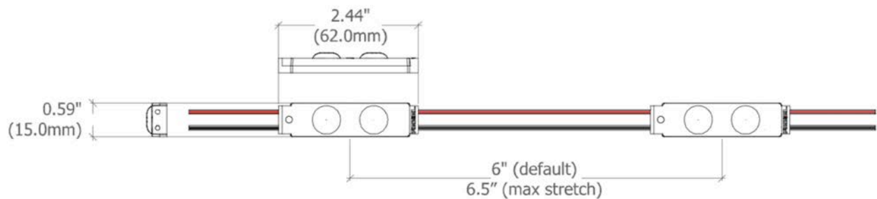
2- Bulb, Small Body, 2 Modules per foot
